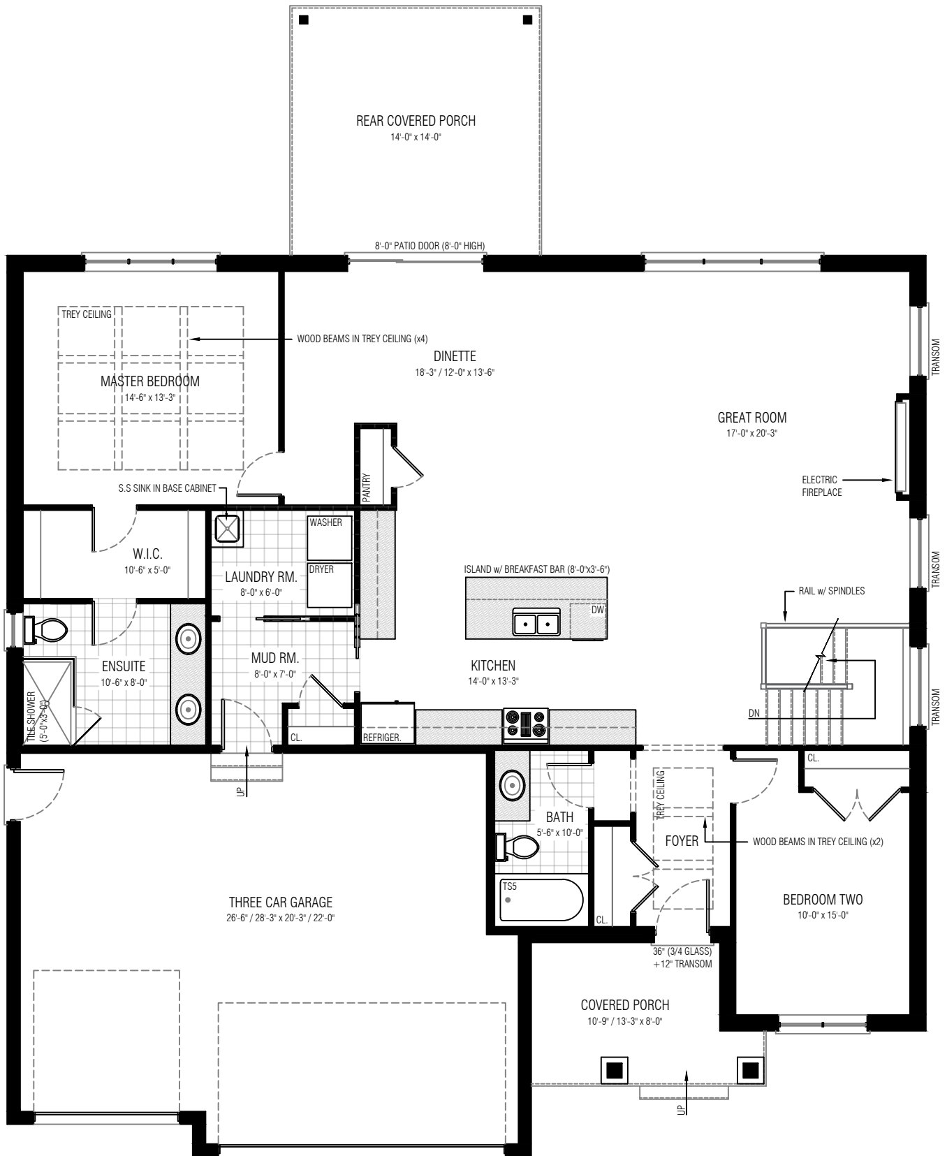
Main Floor Plan (1,800 sq.ft. / 52'-0" x 65'-0" / 9'-0" Ceilings)
